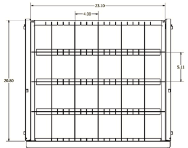
Top View Drawer Layout
